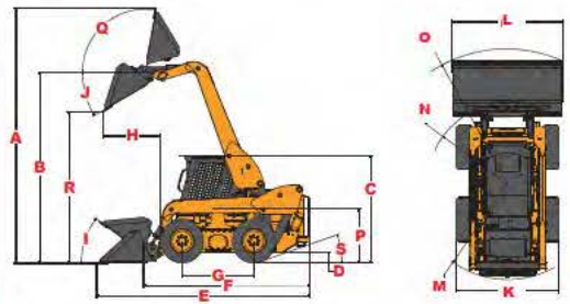
4000V REFERENCE DIAGRAM
