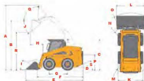
2700V NXT2 / 3300V NXT2 REFERENCE DIAGRAM
